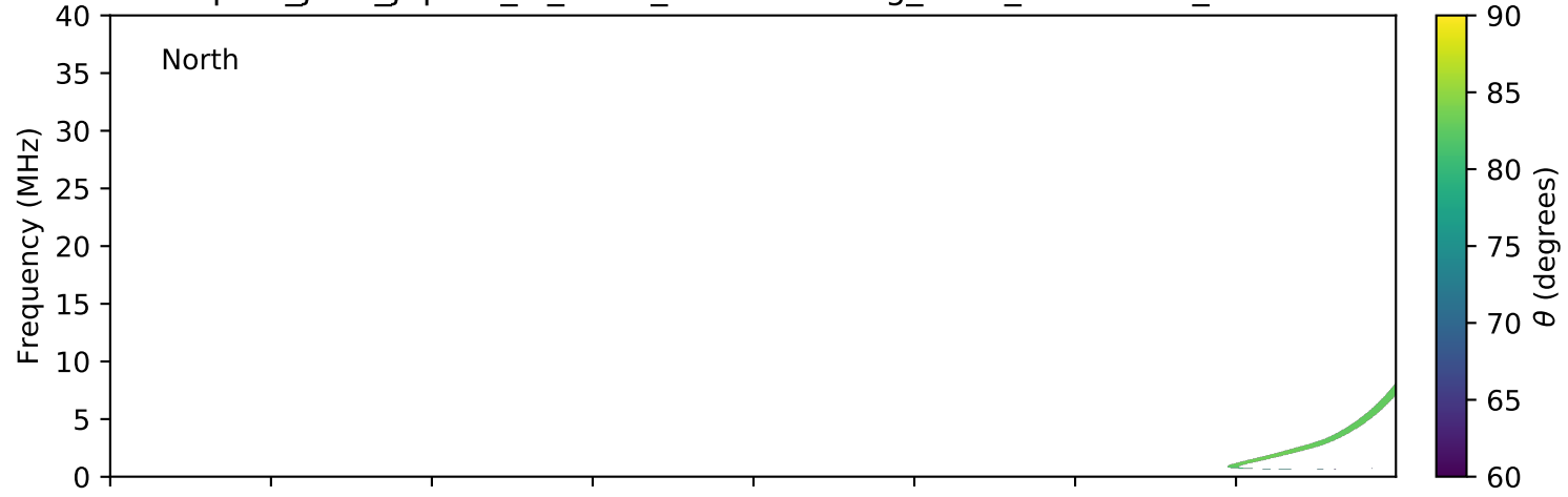
expres_juno_jupiter_io_isaac_lossc-wid1deg_3kev_20180415_v01.cdf
