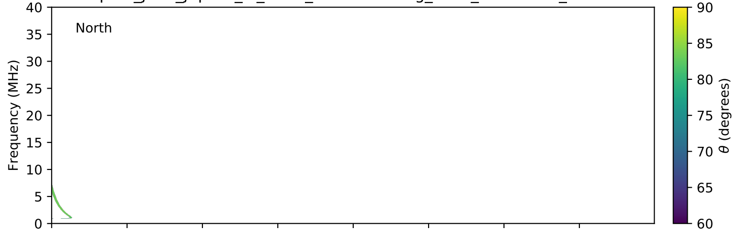
expres_juno_jupiter_io_isaac_lossc-wid1deg_3kev_20180413_v01.cdf
