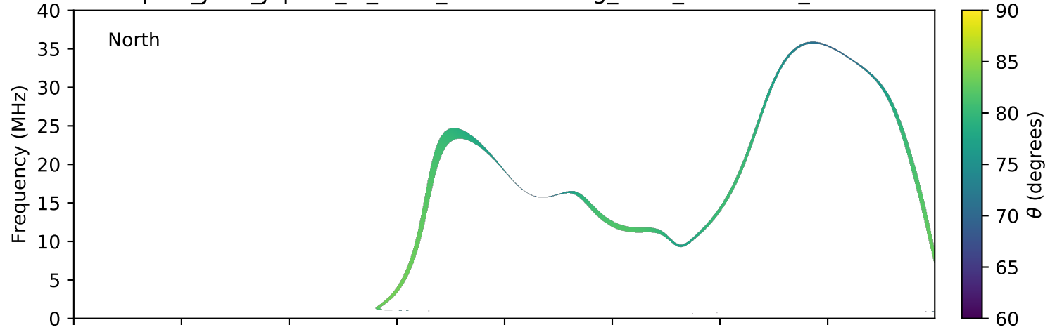
expres_juno_jupiter_io_isaac_lossc-wid1deg_3kev_20180412_v01.cdf
