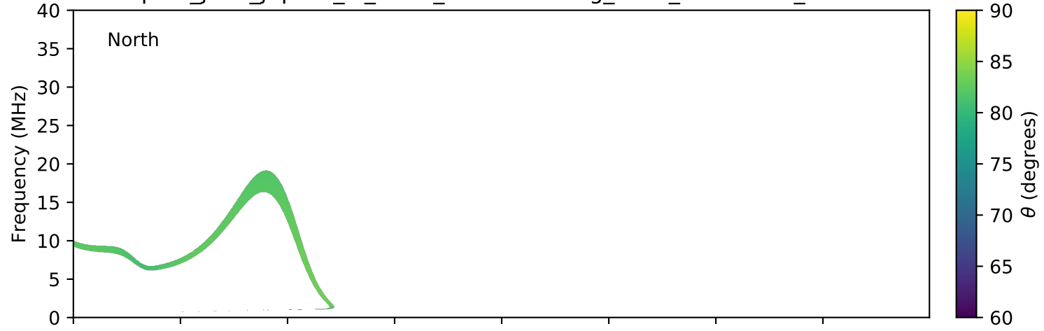
expres_juno_jupiter_io_isaac_lossc-wid1deg_3kev_20180411_v01.cdf
