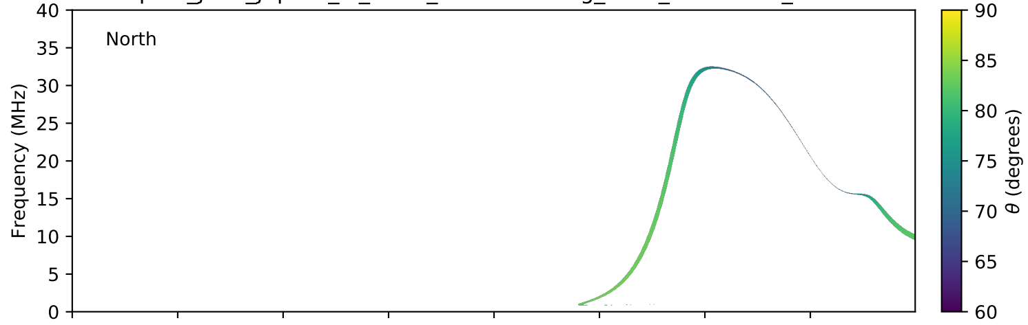
expres_juno_jupiter_io_isaac_lossc-wid1deg_3kev_20180410_v01.cdf
