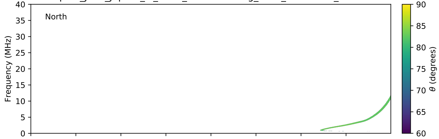
expres_juno_jupiter_io_isaac_lossc-wid1deg_3kev_20180408_v01.cdf
