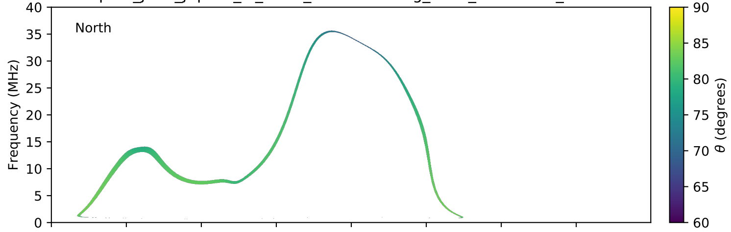
expres_juno_jupiter_io_isaac_lossc-wid1deg_3kev_20180407_v01.cdf
