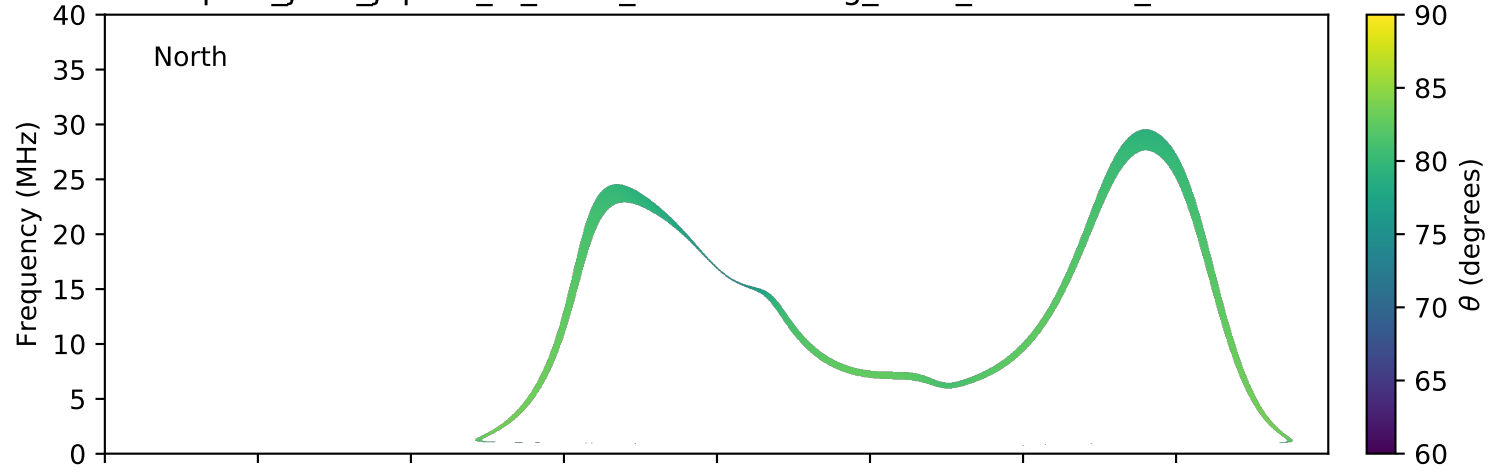
expres_juno_jupiter_io_isaac_lossc-wid1deg_3kev_20180405_v01.cdf
