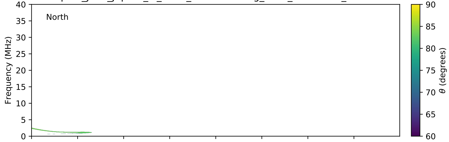
expres_juno_jupiter_io_isaac_lossc-wid1deg_3kev_20180404_v01.cdf
