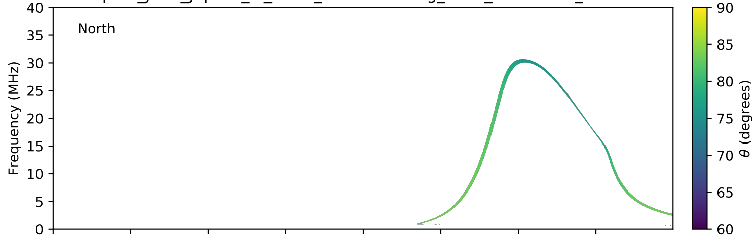
expres_juno_jupiter_io_isaac_lossc-wid1deg_3kev_20180403_v01.cdf
