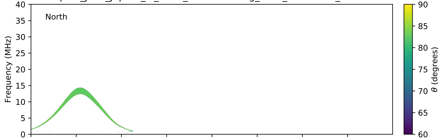
expres_juno_jupiter_io_isaac_lossc-wid1deg_3kev_20180402_v01.cdf
