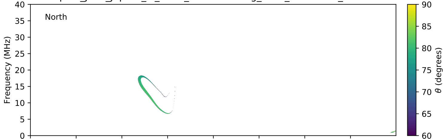
expres_juno_jupiter_io_isaac_lossc-wid1deg_3kev_20180401_v01.cdf
