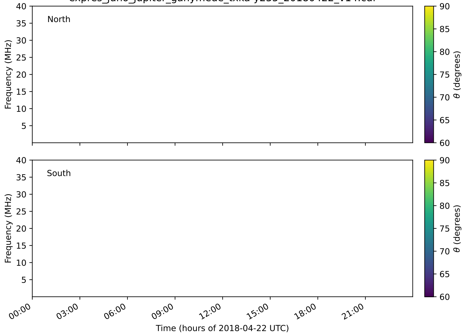
expres_juno_jupiter_ganymede_txka-y235_20180422_v14.cdf
