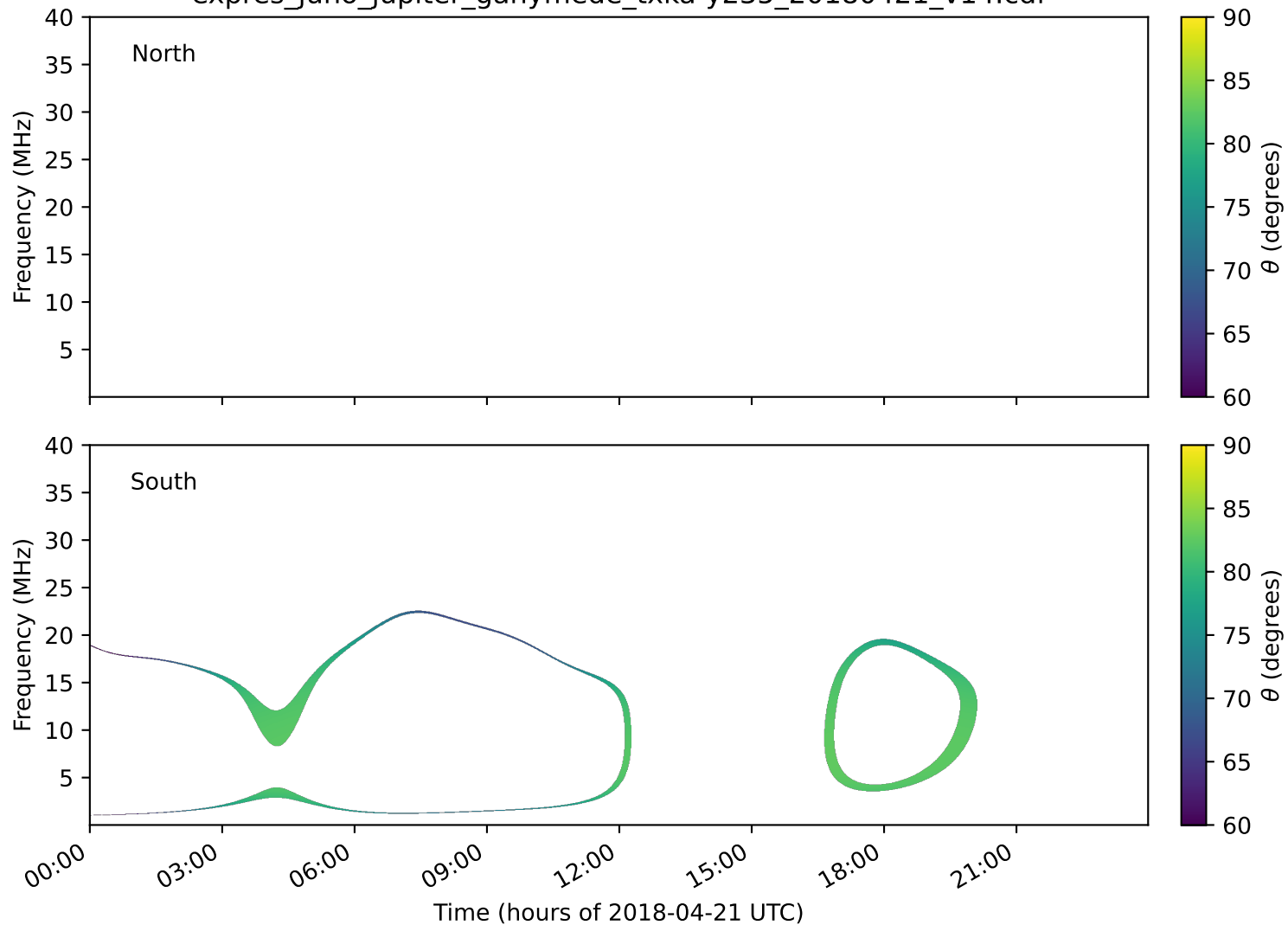
expres_juno_jupiter_ganymede_txka-y235_20180421_v14.cdf
