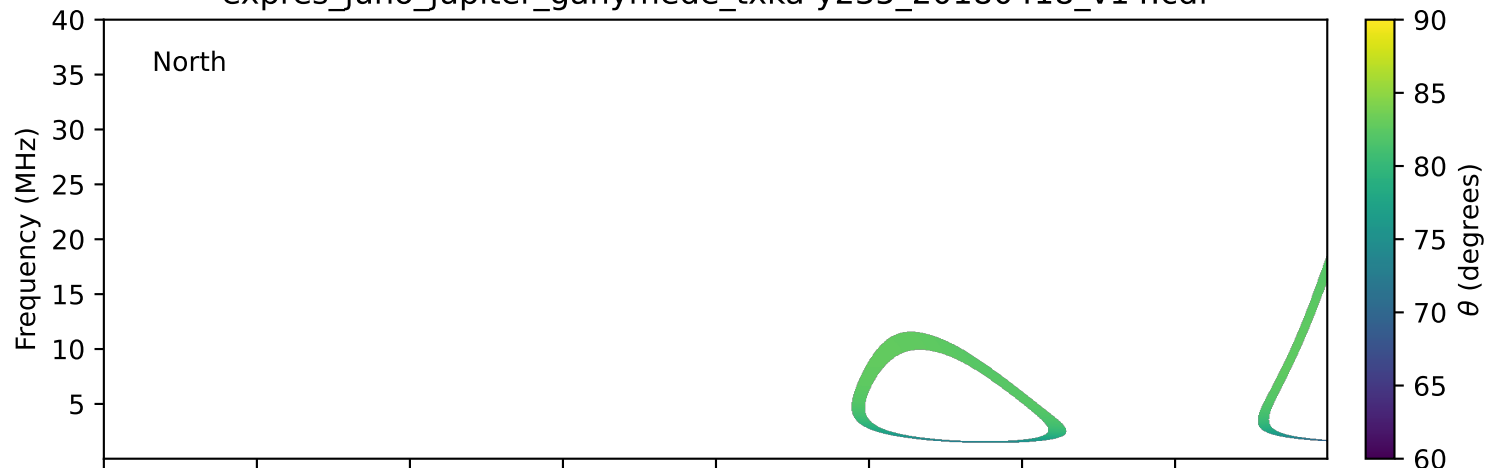
expres_juno_jupiter_ganymede_txka-y235_20180418_v14.cdf
