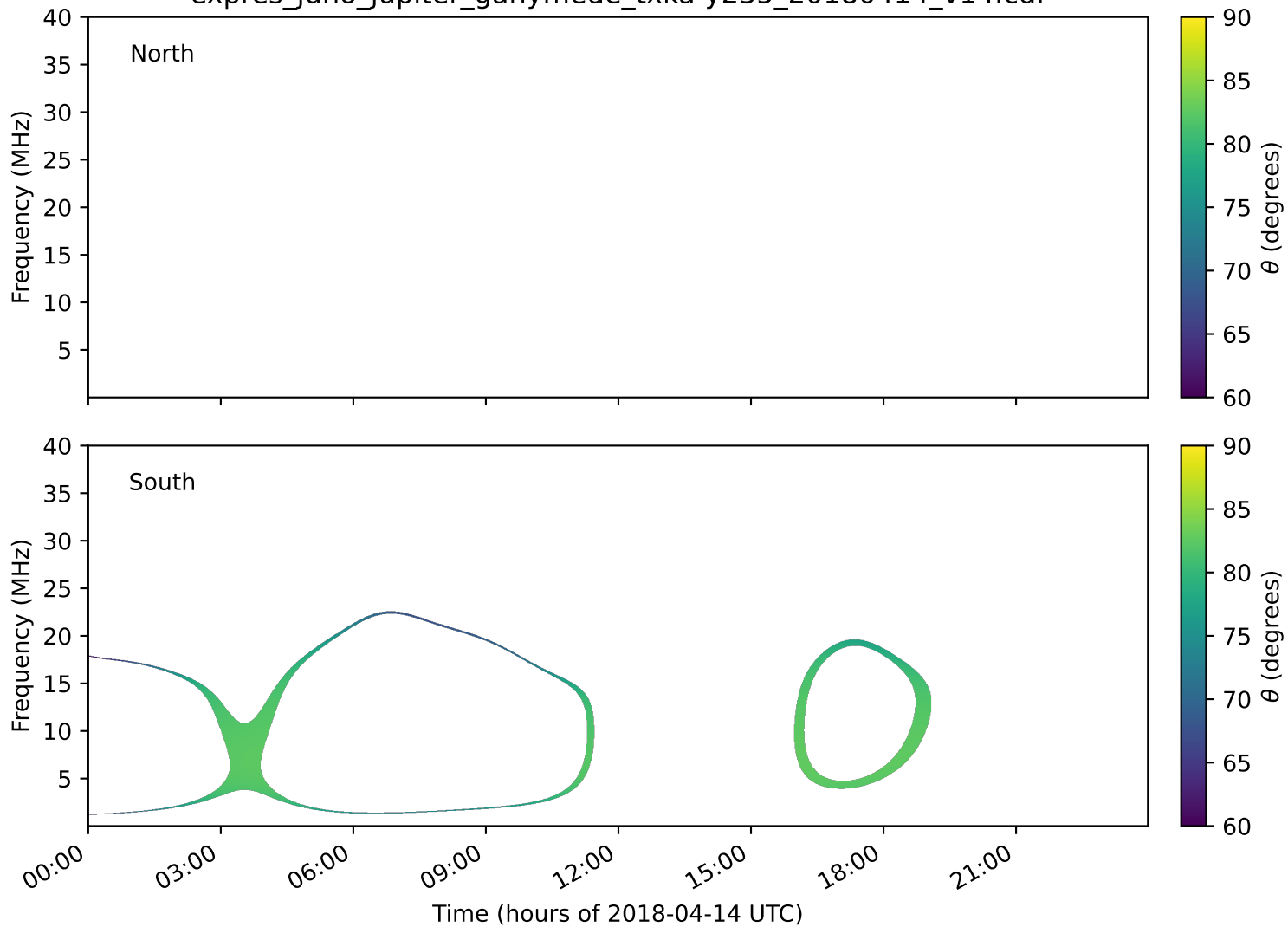
expres_juno_jupiter_ganymede_txka-y235_20180414_v14.cdf
