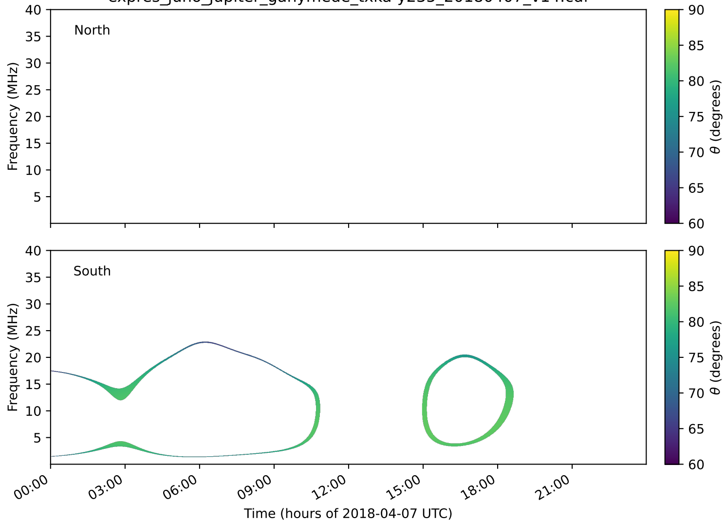
expres_juno_jupiter_ganymede_txka-y235_20180407_v14.cdf
