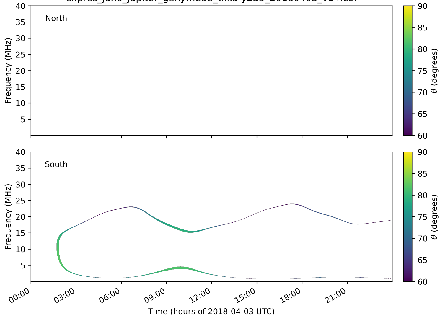
expres_juno_jupiter_ganymede_txka-y235_20180403_v14.cdf
