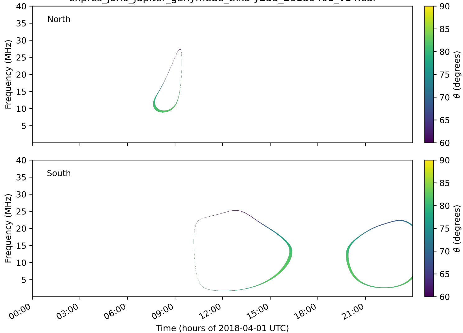
expres_juno_jupiter_ganymede_txka-y235_20180401_v14.cdf
