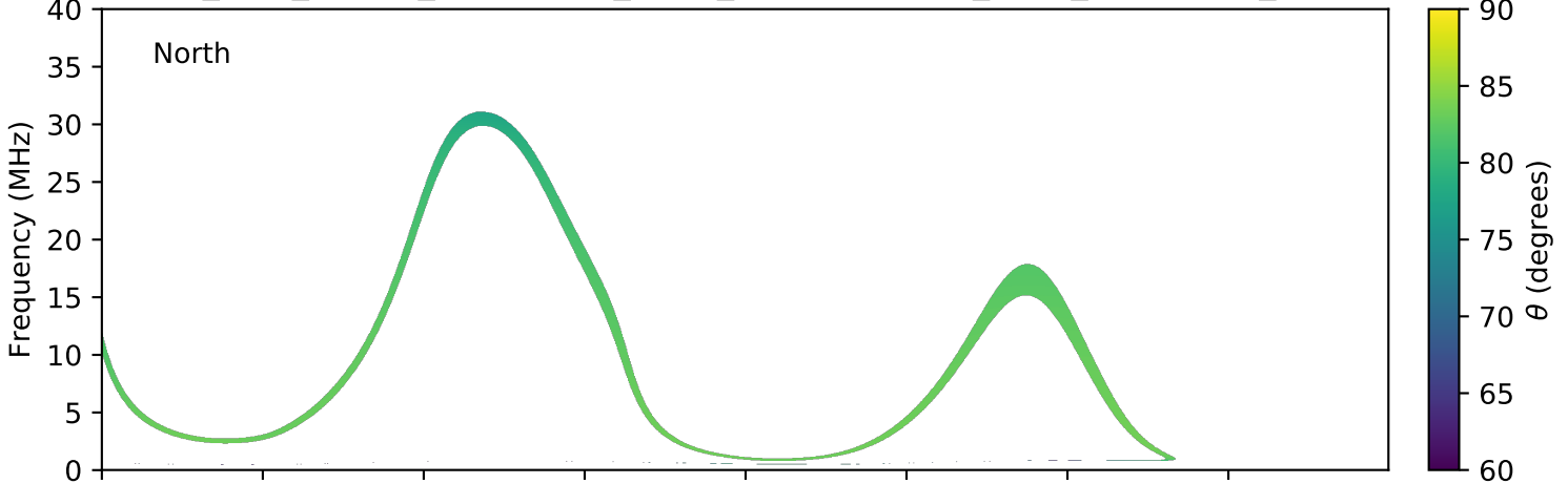
expres_juno_jupiter_ganymede_isaac_lossc-wid1deg_3kev_20180413_v01.cdf
