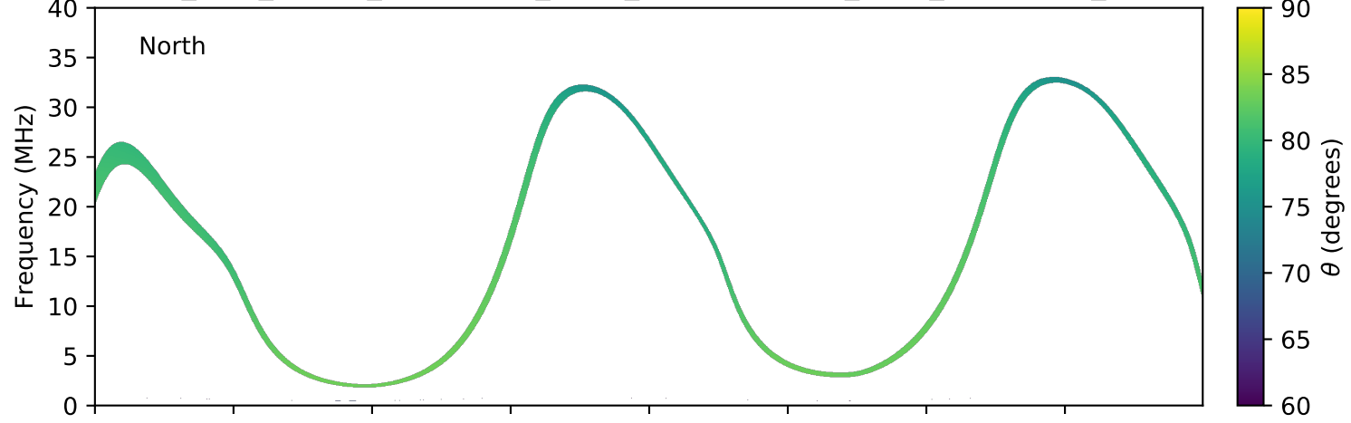
expres_juno_jupiter_ganymede_isaac_lossc-wid1deg_3kev_20180412_v01.cdf
