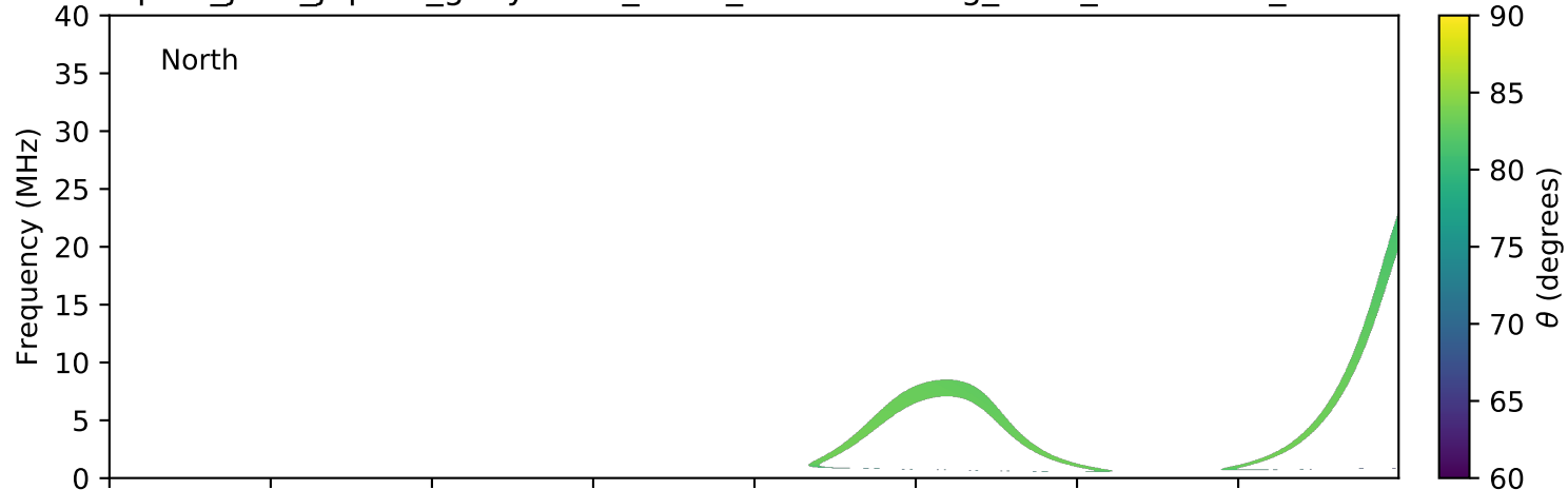
expres_juno_jupiter_ganymede_isaac_lossc-wid1deg_3kev_20180411_v01.cdf
