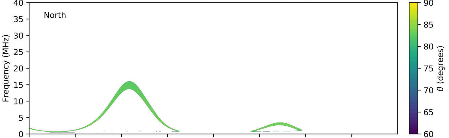
expres_juno_jupiter_ganymede_isaac_lossc-wid1deg_3kev_20180406_v01.cdf
