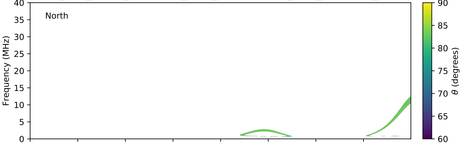
expres_juno_jupiter_ganymede_isaac_lossc-wid1deg_3kev_20180404_v01.cdf
