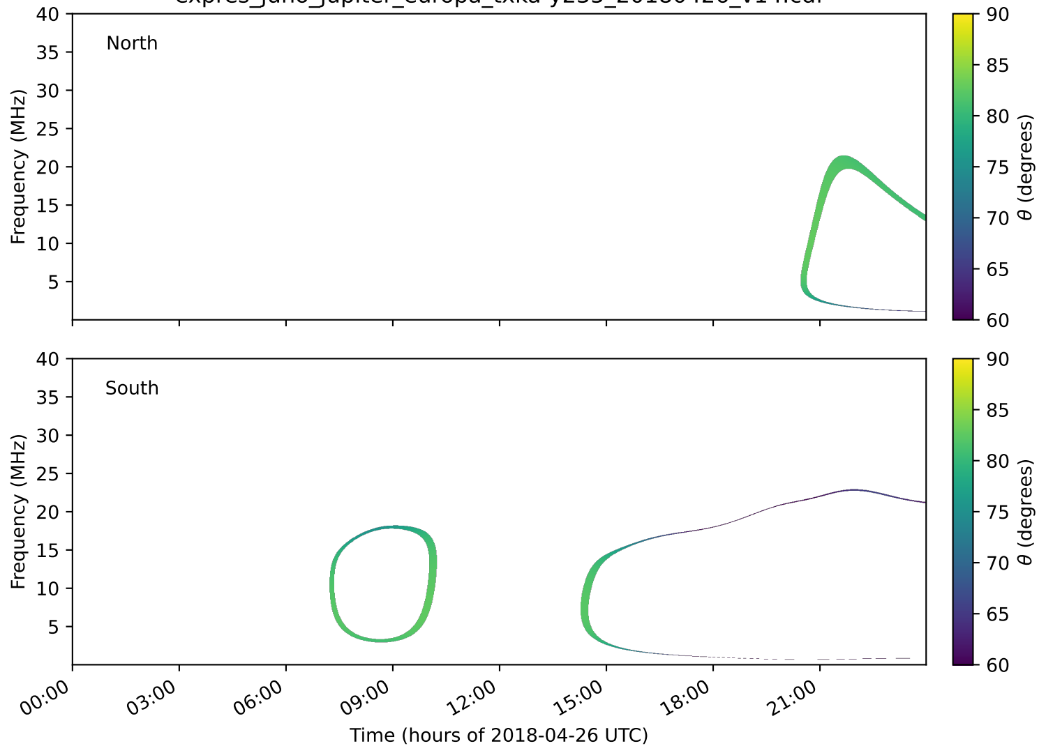
expres_juno_jupiter_europa_txka-y235_20180426_v14.cdf
