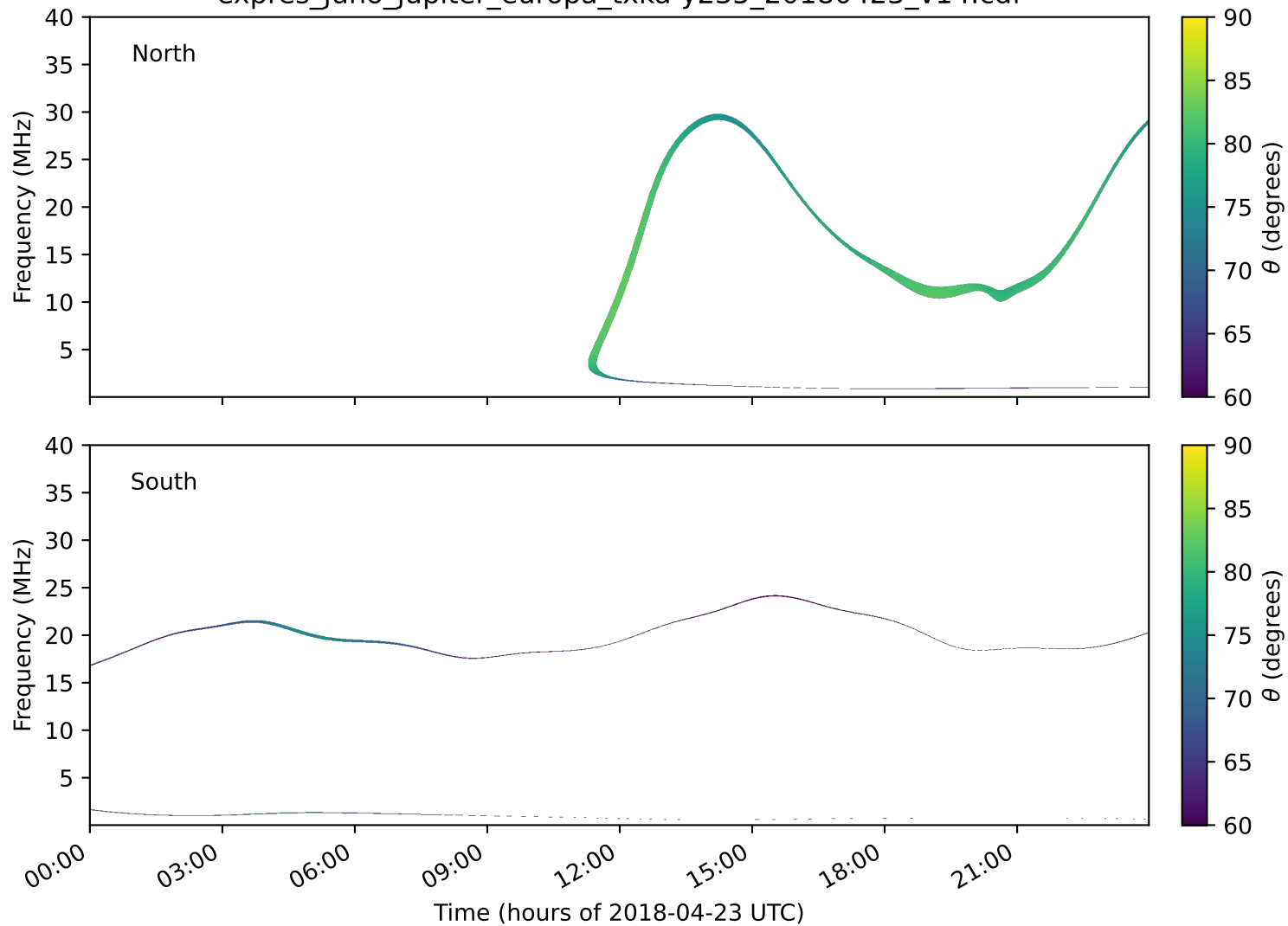
expres_juno_jupiter_europa_txka-y235_20180423_v14.cdf
