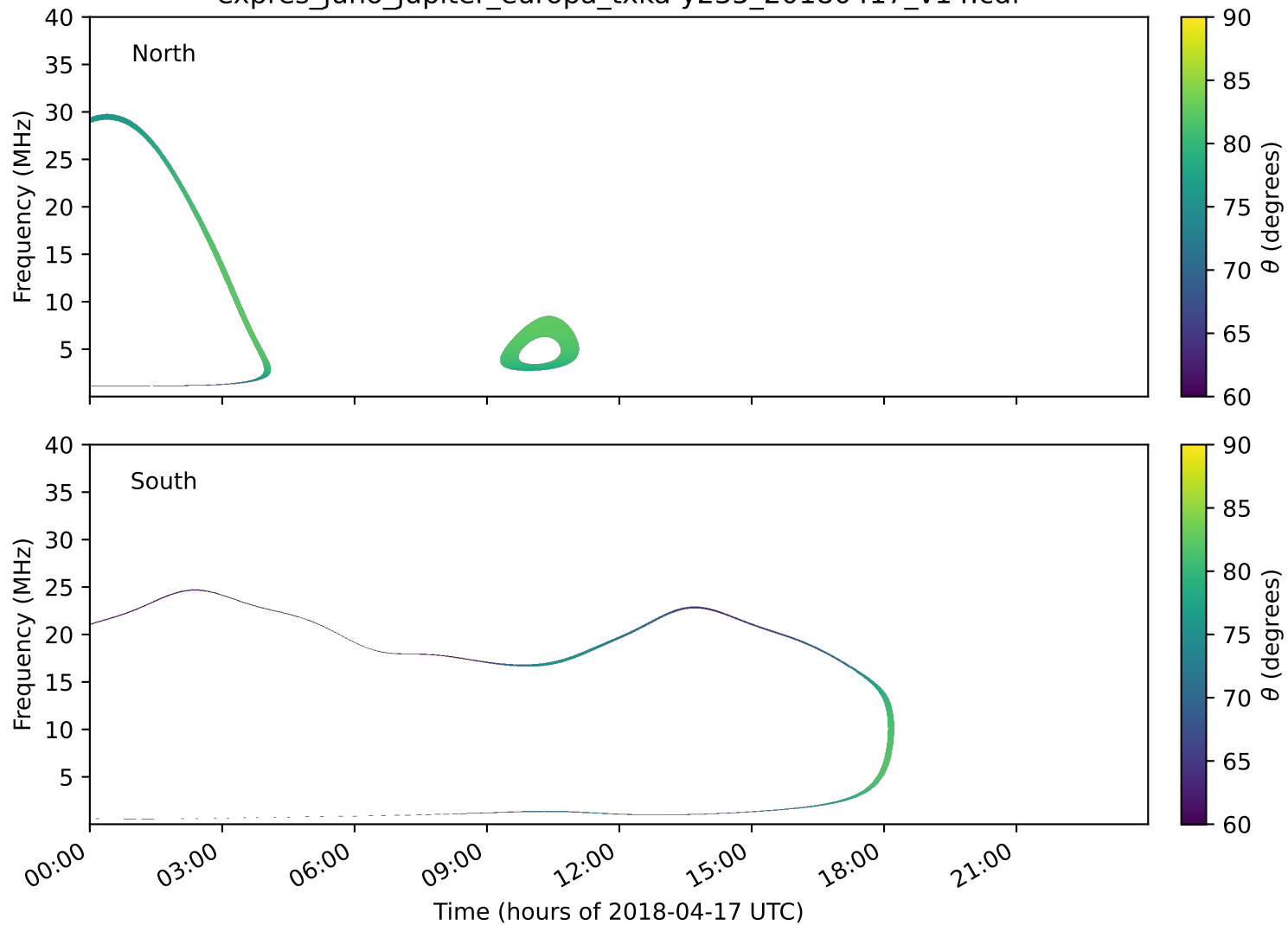
expres_juno_jupiter_europa_txka-y235_20180417_v14.cdf
