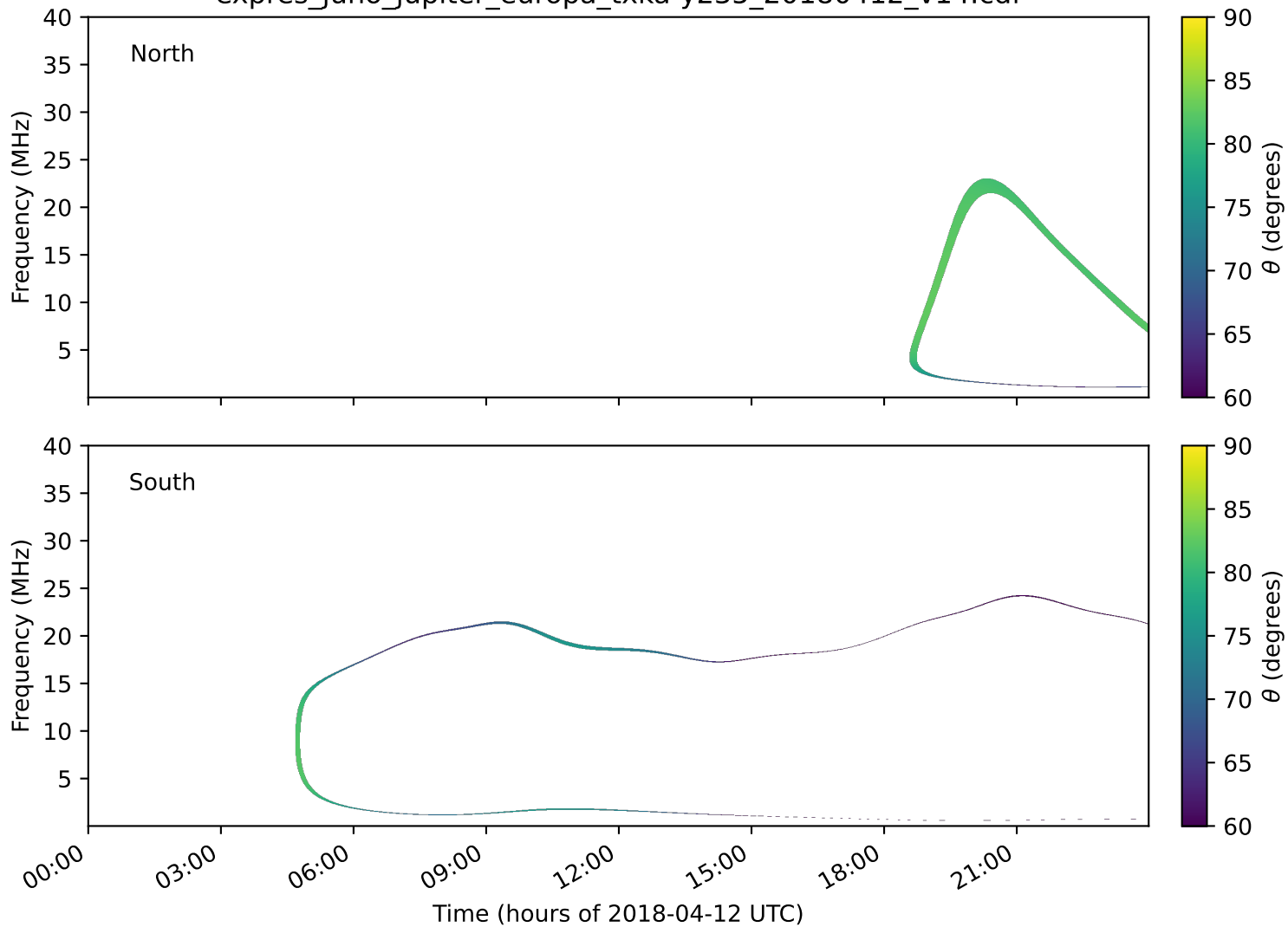
expres_juno_jupiter_europa_txka-y235_20180412_v14.cdf
