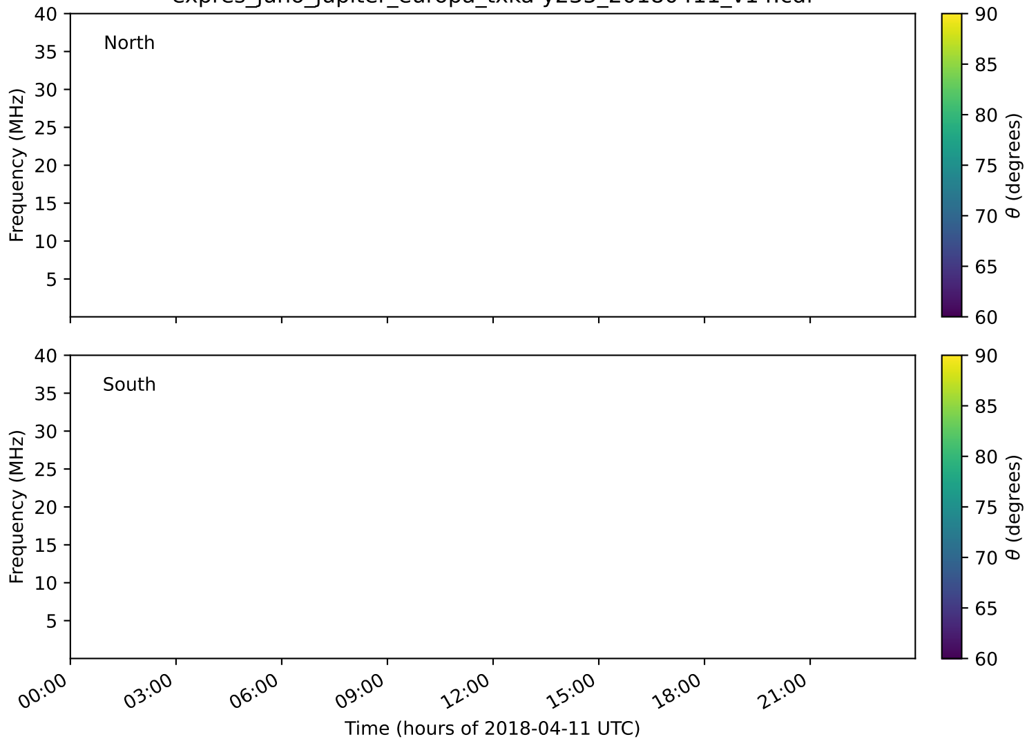
expres_juno_jupiter_europa_txka-y235_20180411_v14.cdf
