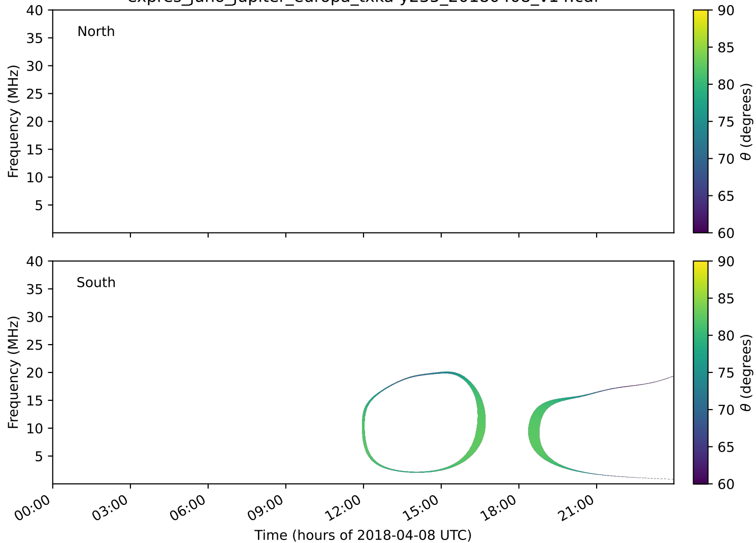
expres_juno_jupiter_europa_txka-y235_20180408_v14.cdf
