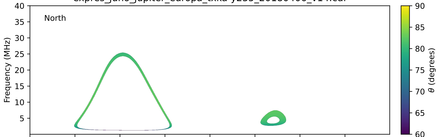
expres_juno_jupiter_europa_txka-y235_20180406_v14.cdf
