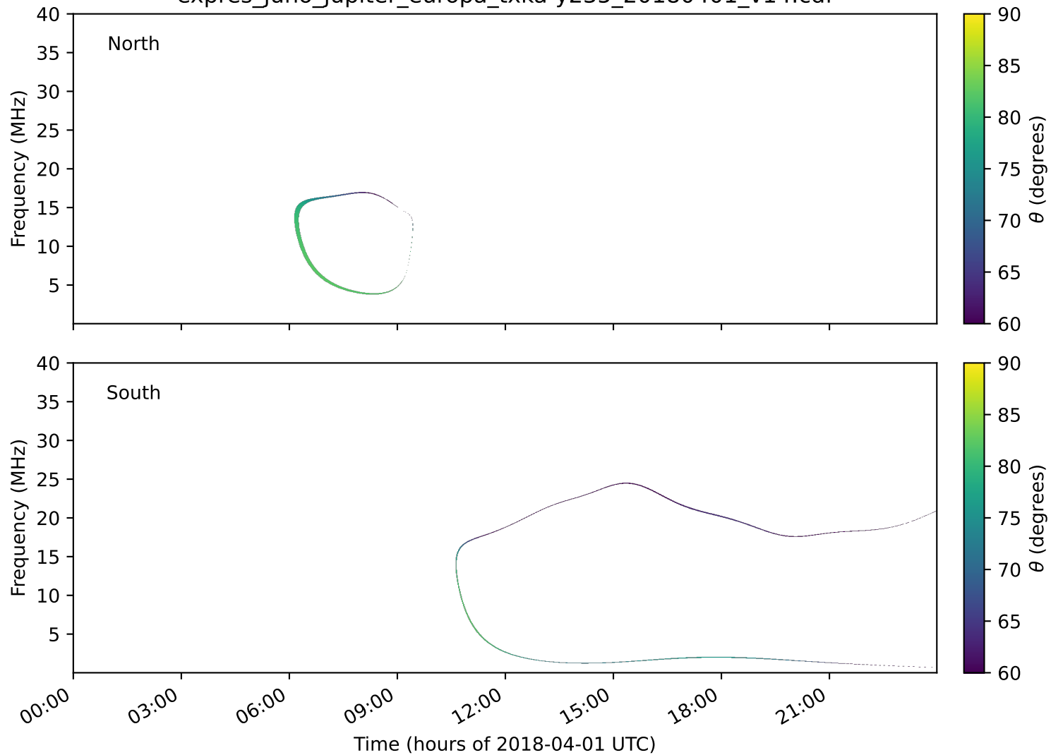
expres_juno_jupiter_europa_txka-y235_20180401_v14.cdf
