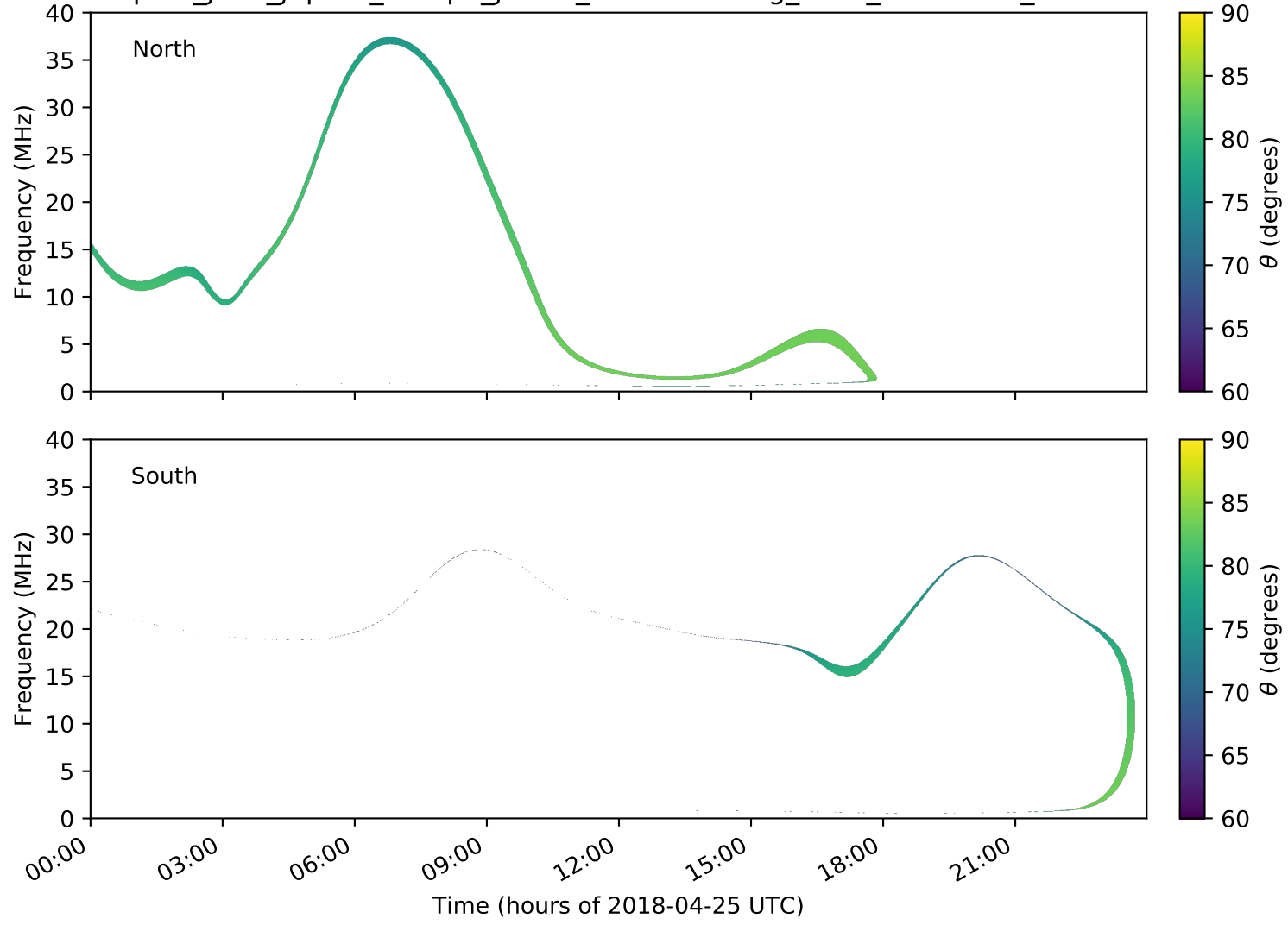
expres_juno_jupiter_europa_jrm09_lossc-wid1deg_3kev_20180425_v01.cdf
