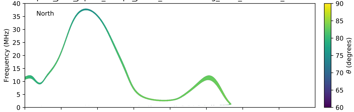
expres_juno_jupiter_europa_jrm09_lossc-wid1deg_3kev_20180423_v01.cdf
