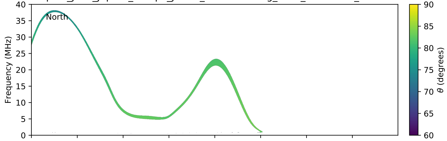
expres_juno_jupiter_europa_jrm09_lossc-wid1deg_3kev_20180419_v01.cdf
