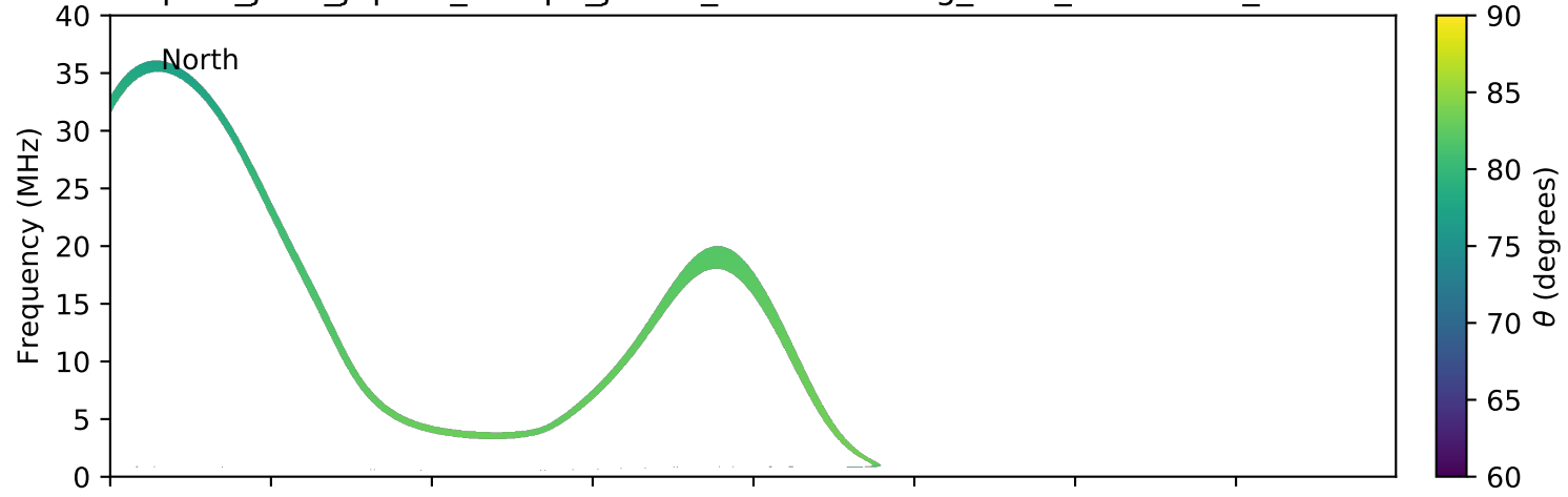
expres_juno_jupiter_europa_jrm09_lossc-wid1deg_3kev_20180412_v01.cdf
