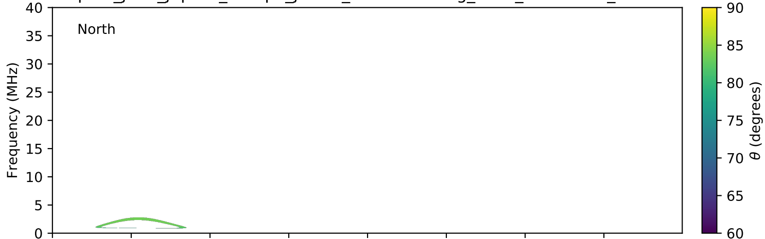
expres_juno_jupiter_europa_jrm09_lossc-wid1deg_3kev_20180402_v01.cdf
