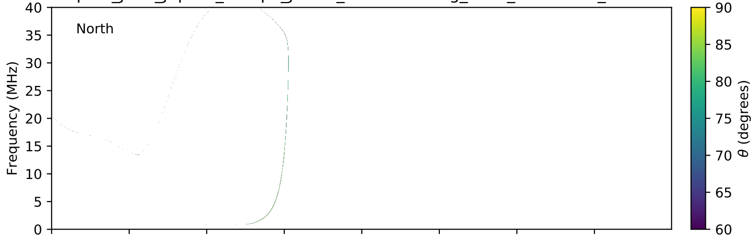
expres_juno_jupiter_europa_jrm09_lossc-wid1deg_3kev_20180401_v01.cdf
