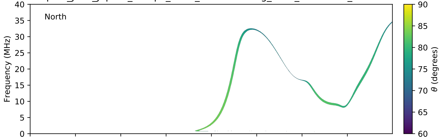
expres_juno_jupiter_europa_isaac_lossc-wid1deg_3kev_20180430_v01.cdf
