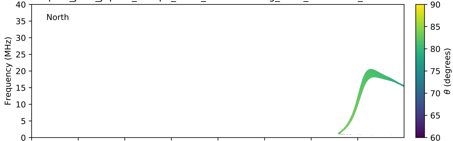
expres_juno_jupiter_europa_isaac_lossc-wid1deg_3kev_20180426_v01.cdf
