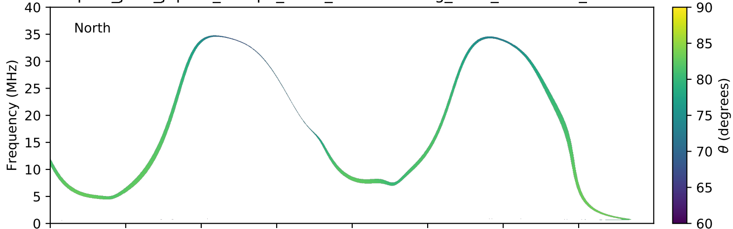
expres_juno_jupiter_europa_isaac_lossc-wid1deg_3kev_20180420_v01.cdf
