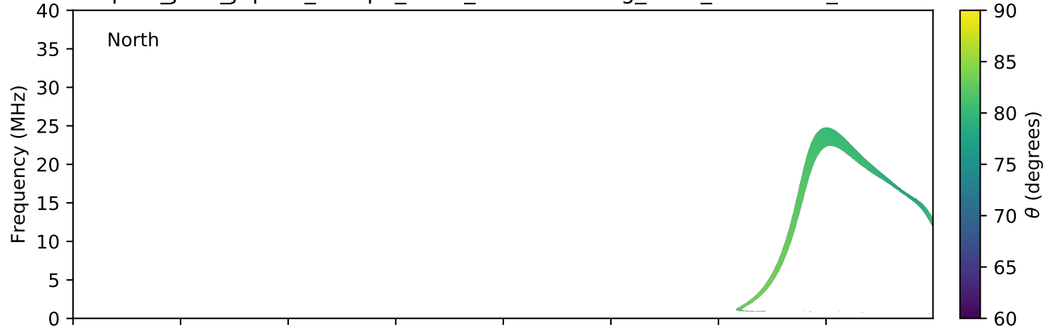
expres_juno_jupiter_europa_isaac_lossc-wid1deg_3kev_20180419_v01.cdf
