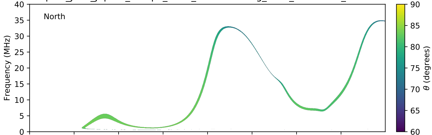
expres_juno_jupiter_europa_isaac_lossc-wid1deg_3kev_20180416_v01.cdf
