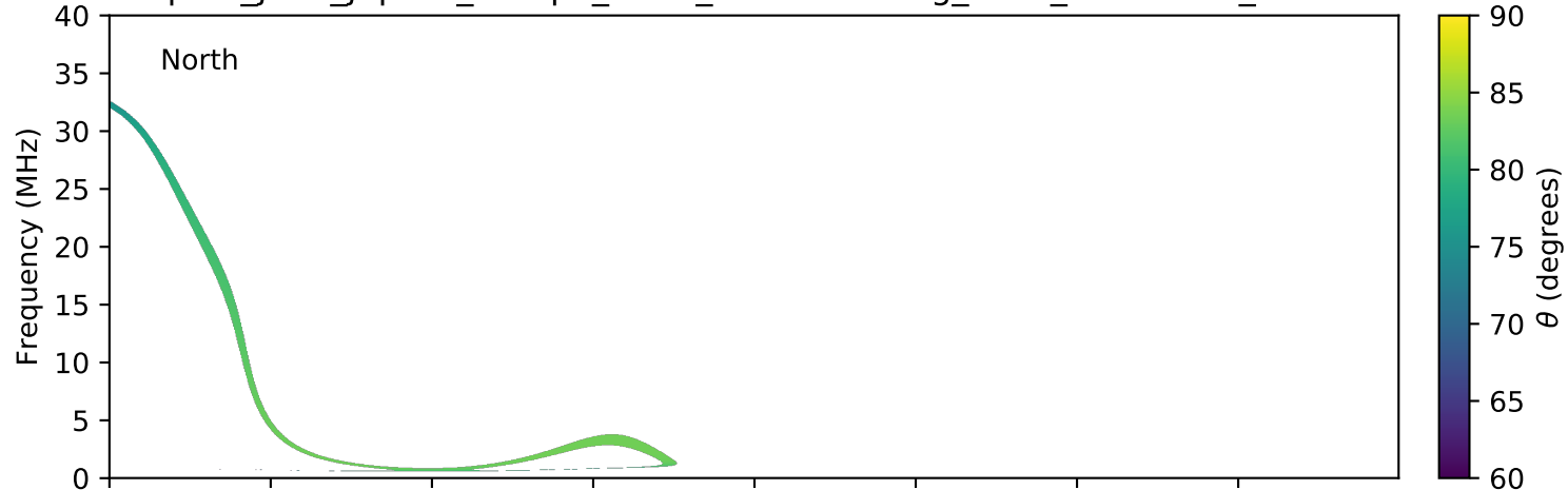
expres_juno_jupiter_europa_isaac_lossc-wid1deg_3kev_20180410_v01.cdf
