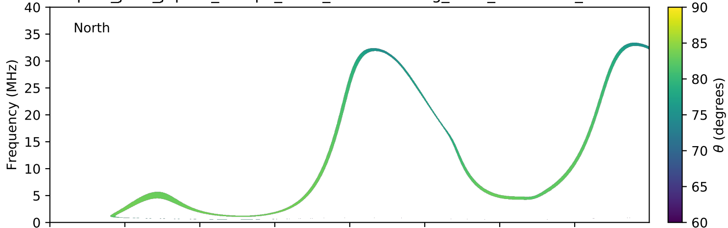
expres_juno_jupiter_europa_isaac_lossc-wid1deg_3kev_20180409_v01.cdf
