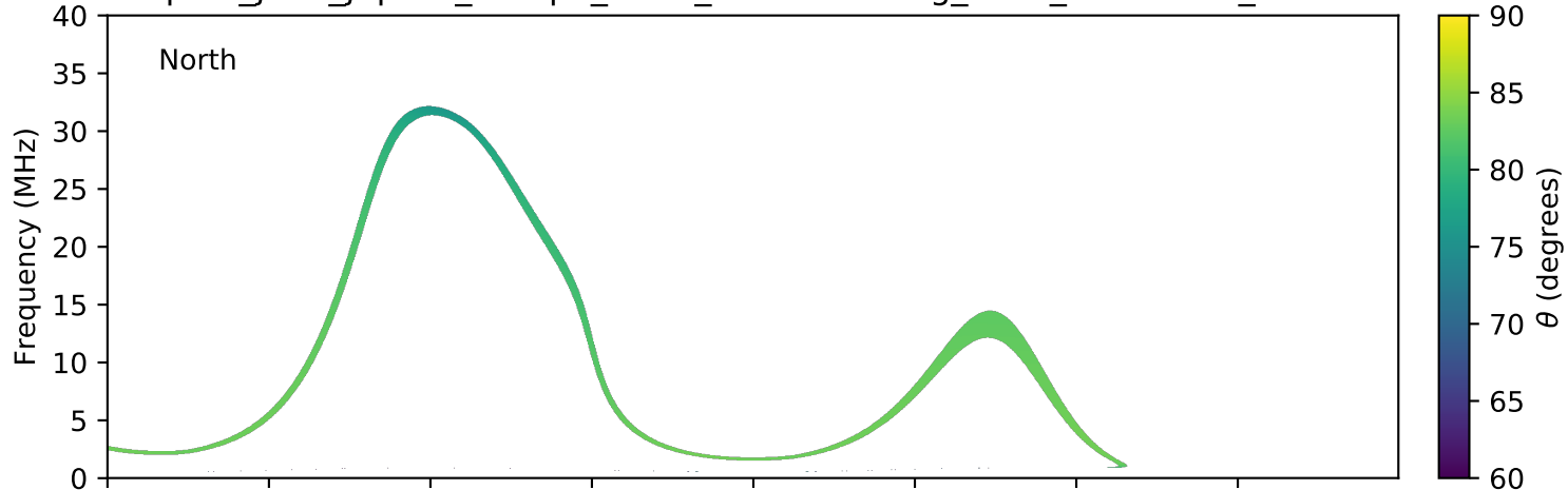
expres_juno_jupiter_europa_isaac_lossc-wid1deg_3kev_20180406_v01.cdf
