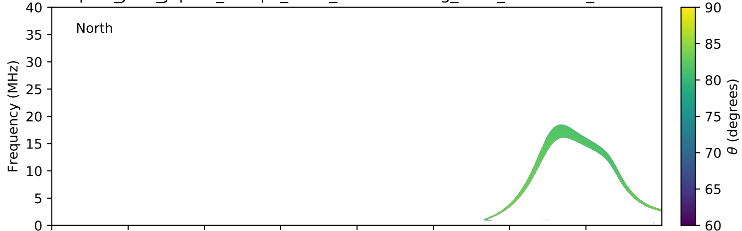
expres_juno_jupiter_europa_isaac_lossc-wid1deg_3kev_20180405_v01.cdf
