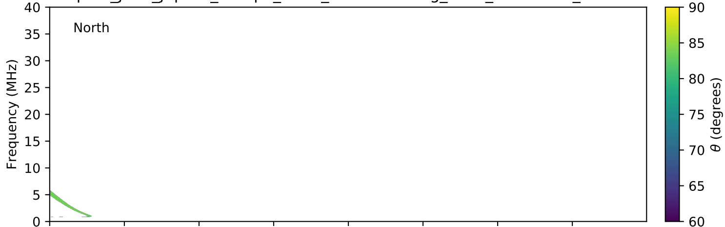
expres_juno_jupiter_europa_isaac_lossc-wid1deg_3kev_20180403_v01.cdf
