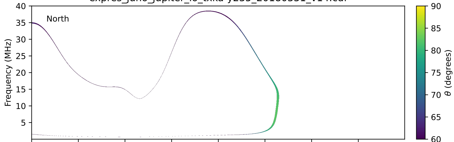
expres_juno_jupiter_io_txka-y235_20180331_v14.cdf
