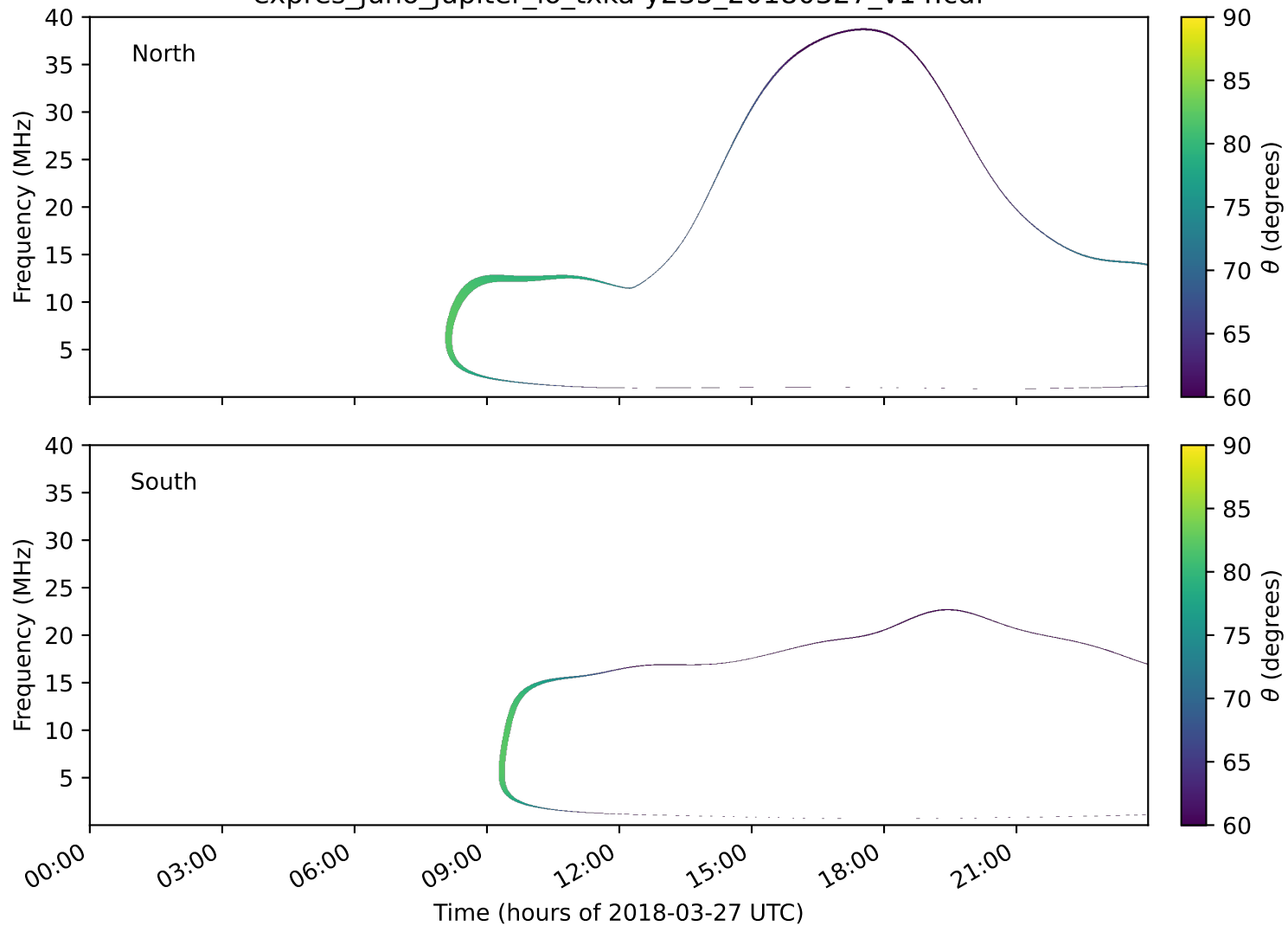
expres_juno_jupiter_io_txka-y235_20180327_v14.cdf
